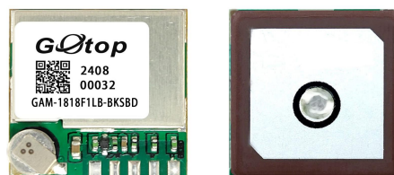
产品图：GAM-1818F1LB-BKSBD
