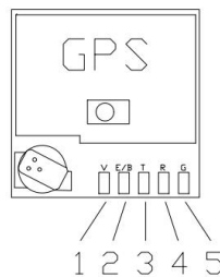
Figure 2: Pin Assignment
