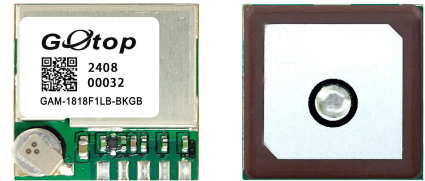
Figure: GAM-1818F1LB-BKGB Top View
