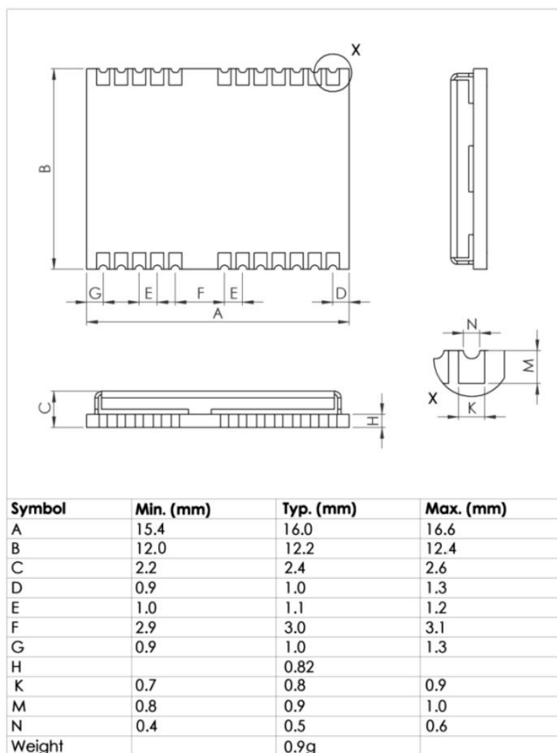
Figure 6: Top view Dimensions
