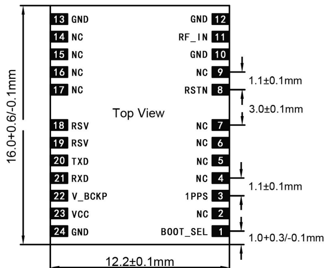
Figure 2: Pin Assignment
