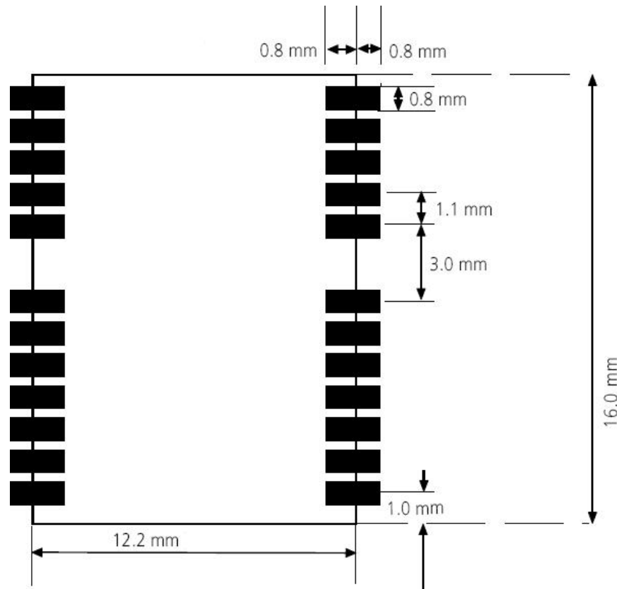
Figure 6: Top view Dimensions
