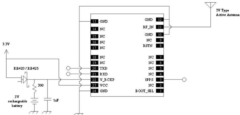
Figure 3: Application Circuit
