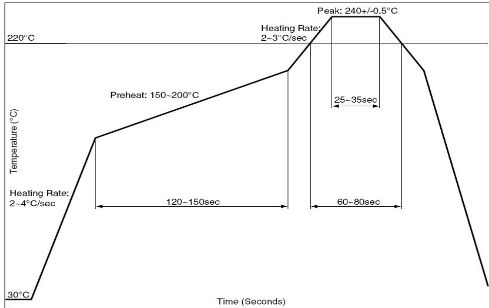
Figure 7: Recommended Reflow Soldering Thermal Profile
